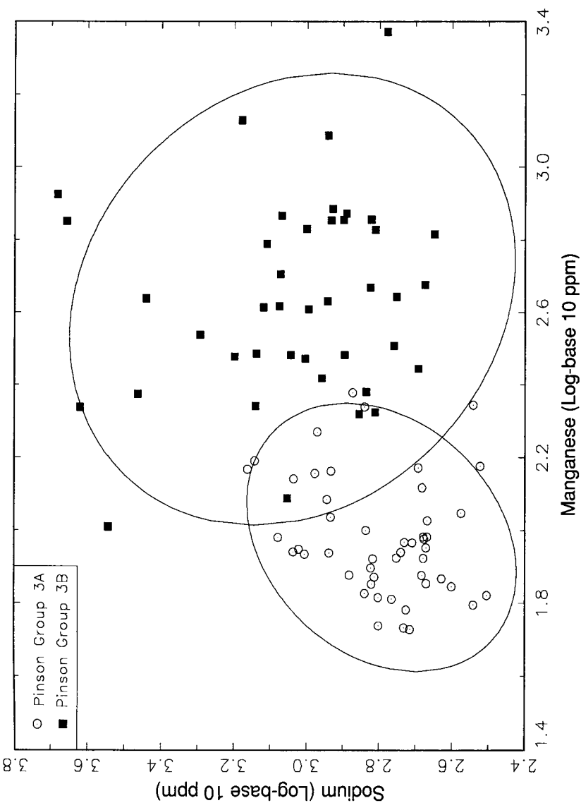
Figure 5. Plot of \log_{10} concentrations of manganese vs. sodium, groups 3A and 3B.
