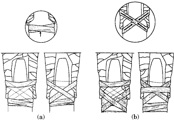
Figure 11. Cross-hatched sinew binding patterns. (a) Upper, tuck loose end under wrap; (b) upper, directions of force application to binding when pressure is placed on edge of point.
