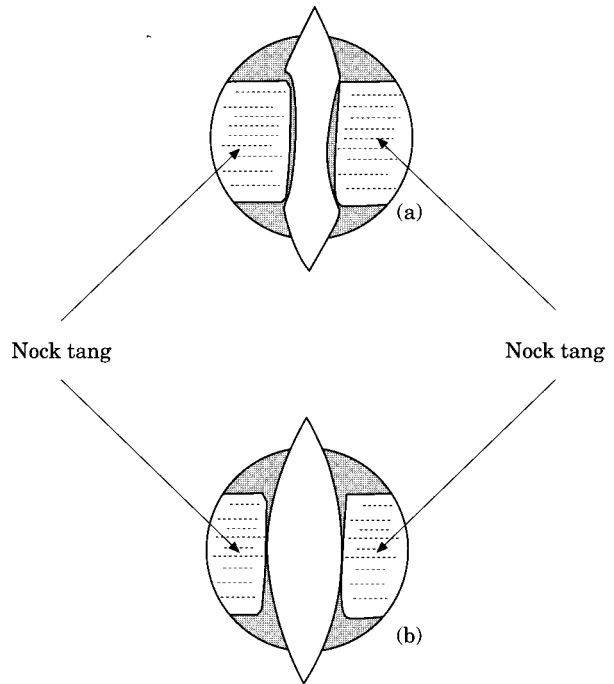
Figure 9. Distal view of the cross section of a fluted (a) and non-fluted biface (b) seated in a notched shaft. Note that the nock tangs are thicker in the former than in the latter and that the nock tangs are within the flute. Pressure to a point edge would cause the unfluted biface to slip within the nock; the fluted point will slip much less, if at all, because the stone tool is wider at the edge of the flute scar than the nock.
