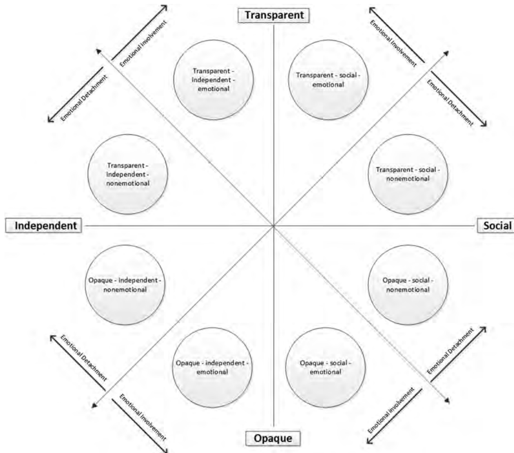
Figure 1 (Garcia et al.). Graph 1: A tentative reformulation of behavioral types that includes emotions.
